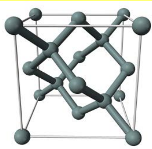
Fig. 66. Silicon crystal lattice
