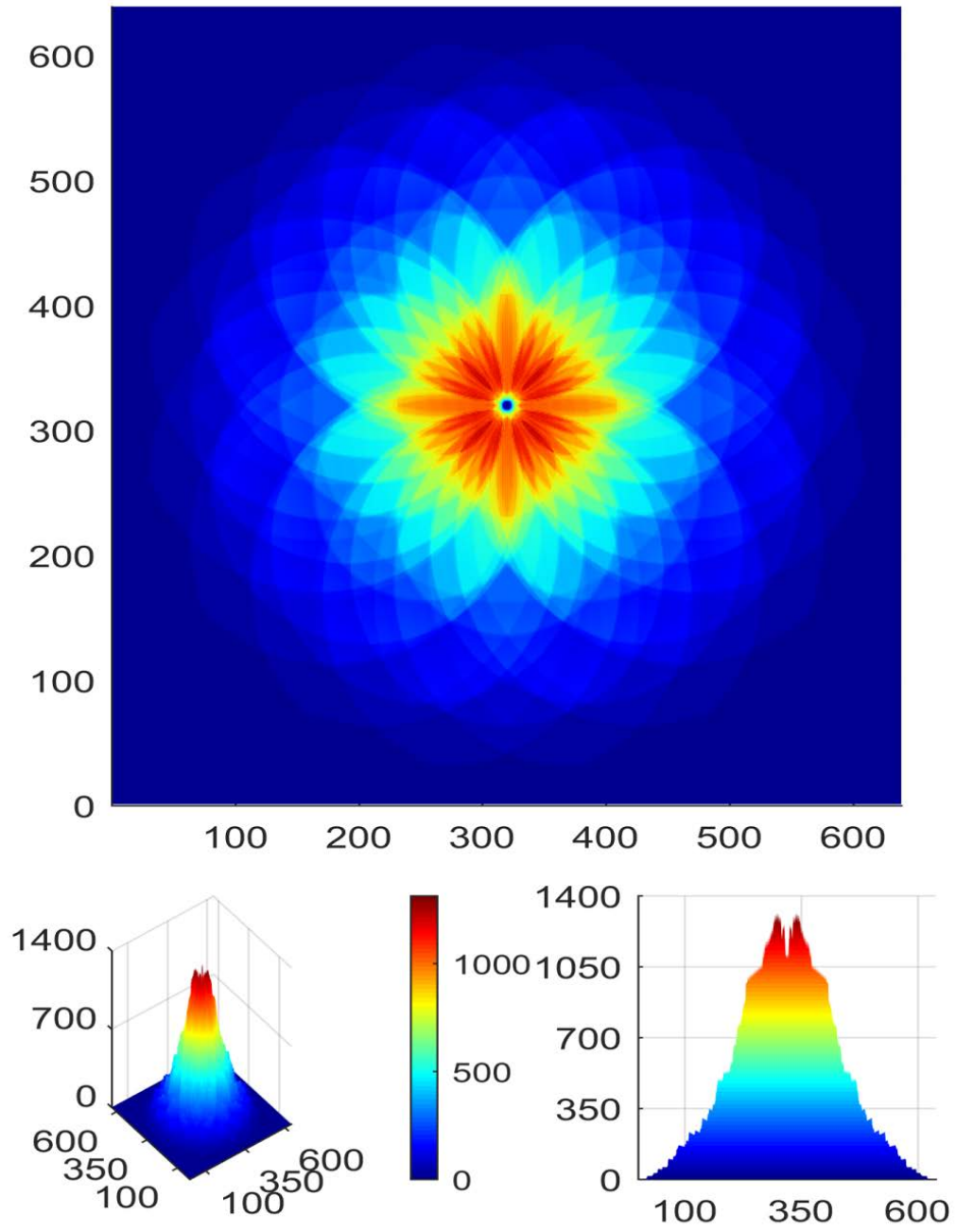
Fig.21. The distribution of the field intensity I over the resonator in the 3rd stage of calculations at a height of h = 24 \mu\text{m} in different projections, range I = 0.008 \div 1314.52 \text{ (W/m}^2\text{)}
