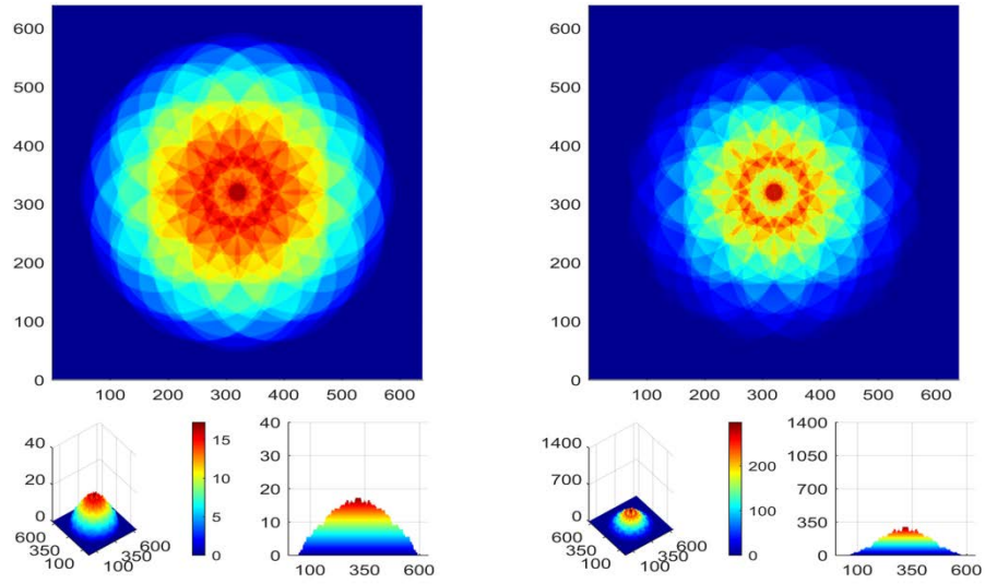
Fig.31. Strength E (on the left) and intensity I (on the right) at level 160h (3.84 mm)
