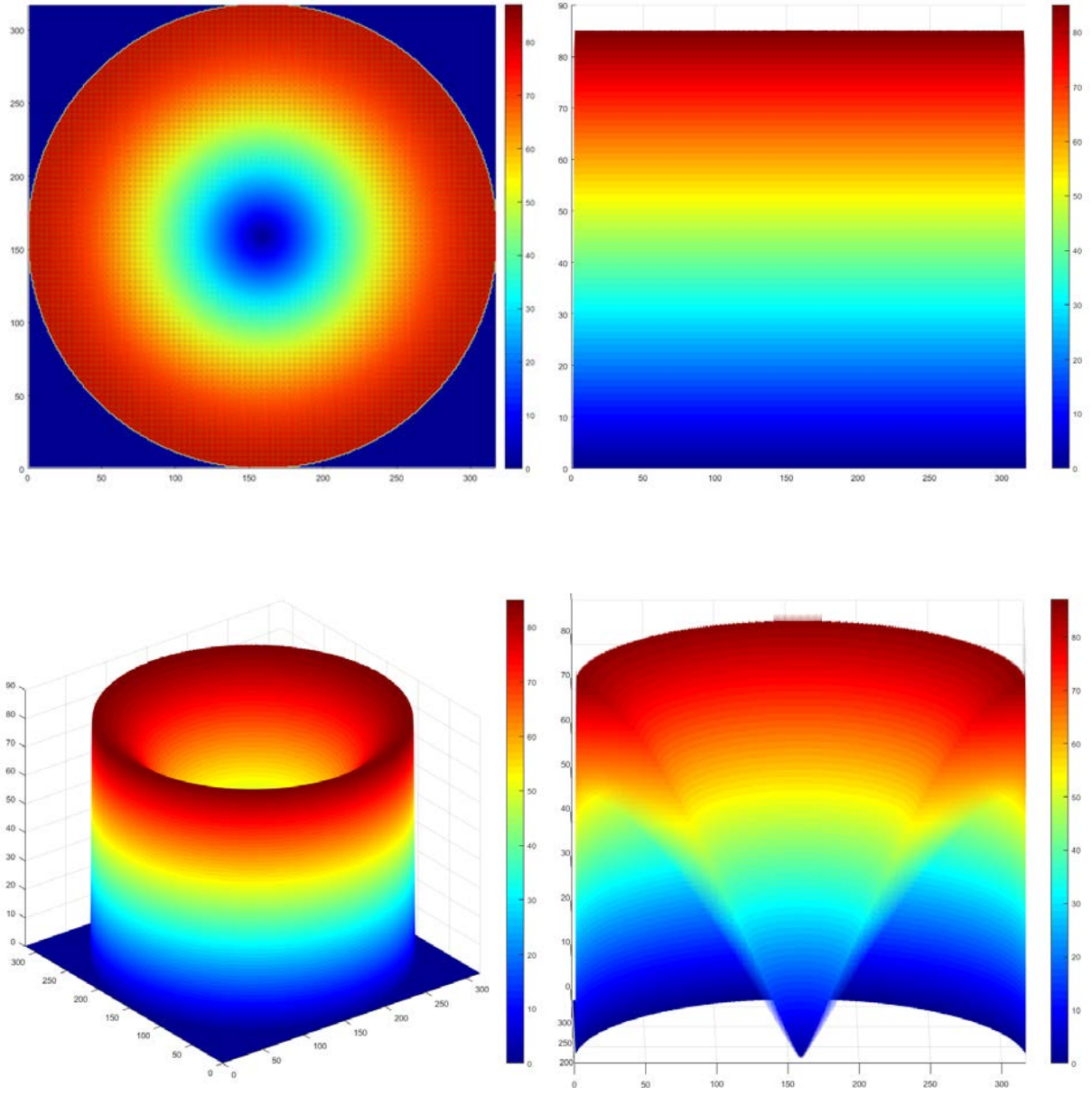
Fig. 9. The distribution of the field strength E over the resonator in the 2nd stage of calculations (horizontal section at a height of h = 24 \mu\text{m} ), range E = 1.02 \div 85.36 \text{ (V/m)}
