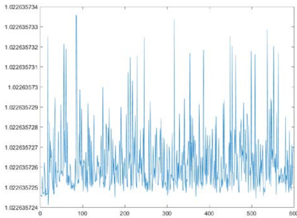
Fig. 50. Graph of field strength over time E(T) , \Delta t = 10^{-3}s
