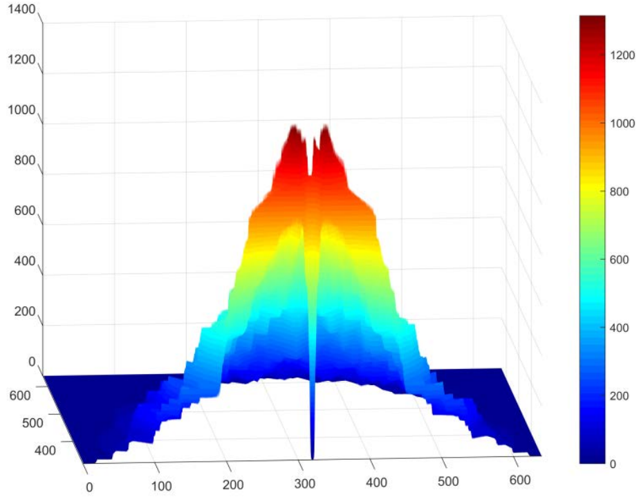
Fig. 22. The distribution of the field intensity I over the resonator at a height of h = 24 \mu\text{m} . Central section.
