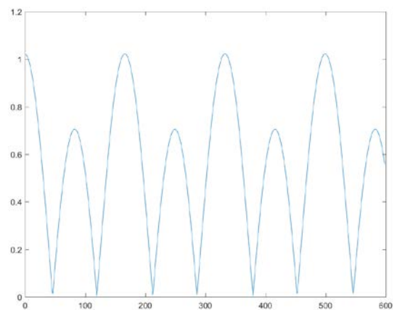
Fig. 59. Graph of field strength over time E(T) , \Delta t = 10^{-12} s , frequency \nu_1 = 6.85 GHz, frequency \nu_2 = 5.38 GHz
