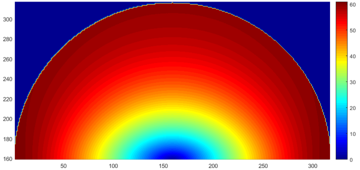
Fig.5. The distribution of the field strength E (V/m) over the resonator in the 1st stage of calculations (vertical section through the center)
