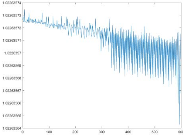
Fig. 48. Graph of field strength over time E(T) , \Delta t = 0.1s
