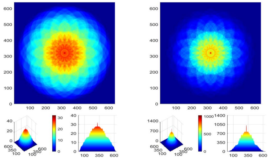
Fig.27. Strength E (on the left) and intensity I (on the right) at level 80h (1.92 mm)
