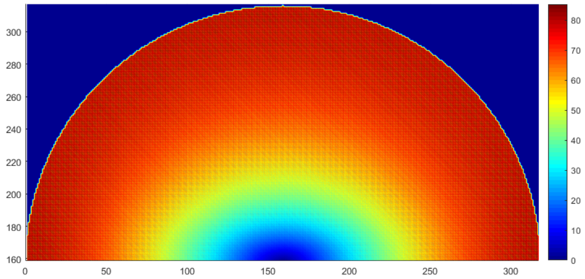
Fig.7. The distribution of the field strength E (V/m) over the resonator in the 2nd stage of calculations (vertical section through the center)
