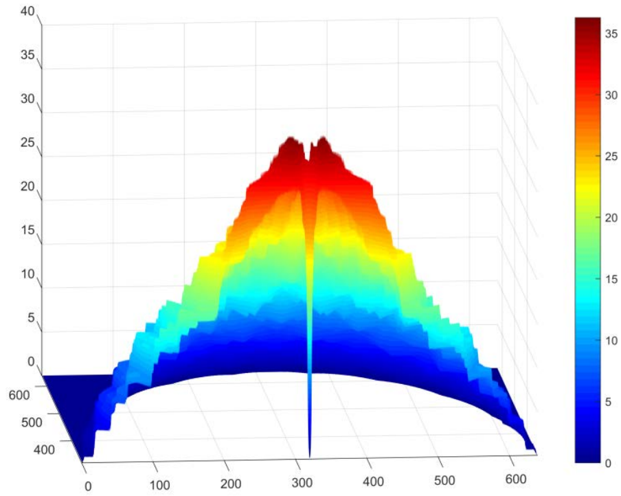
Fig. 19. The distribution of the field strength E over the resonator at a height of h = 24 \mu\text{m} . Central section.
