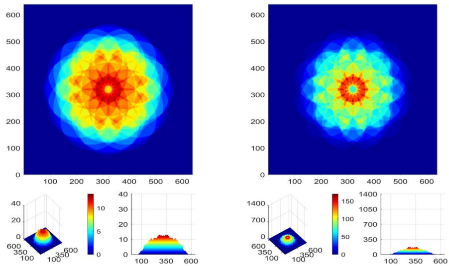
Fig.33. Strength E (on the left) and intensity I (on the right) at level 200h (4.8 mm)
