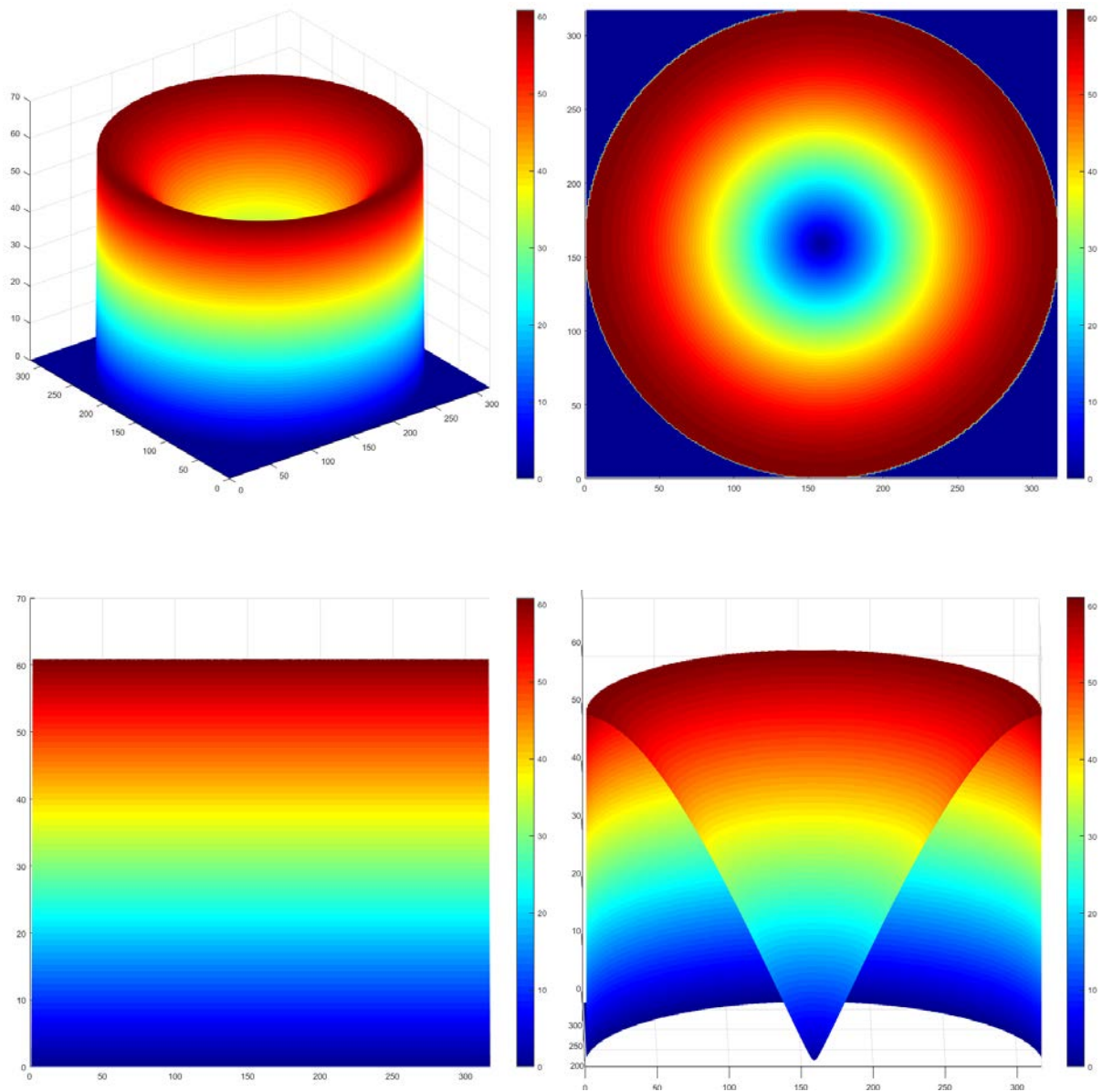
Fig. 6. The distribution of the field strength E over the resonator in the 1st stage of calculations (horizontal section at a height of h = 24 \mu\text{m} ), range E = 1.02 \div 61.08 \text{ (V/m)}
