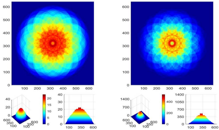
Fig.29. Strength E (on the left) and intensity I (on the right) at level 120h (2.88 mm)
