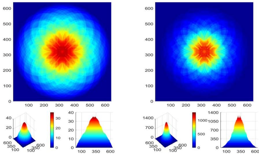
Fig.24. Strength E (on the left) and intensity I (on the right) at level 20h (0.48 mm)
