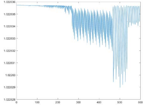
Fig. 47. Graph of field strength over time E(T) , \Delta t = 1s
