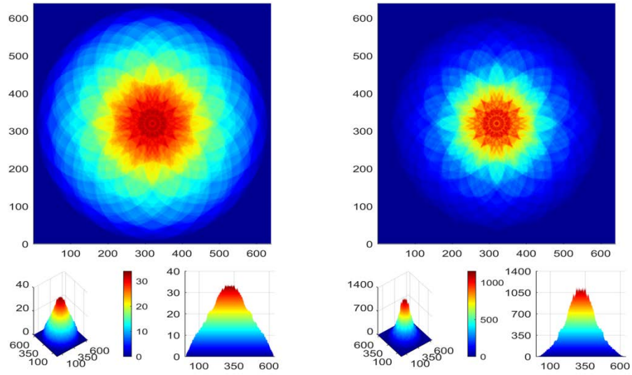
Fig.25. Strength E (on the left) and intensity I (on the right) at level 40h (0.96 mm)
