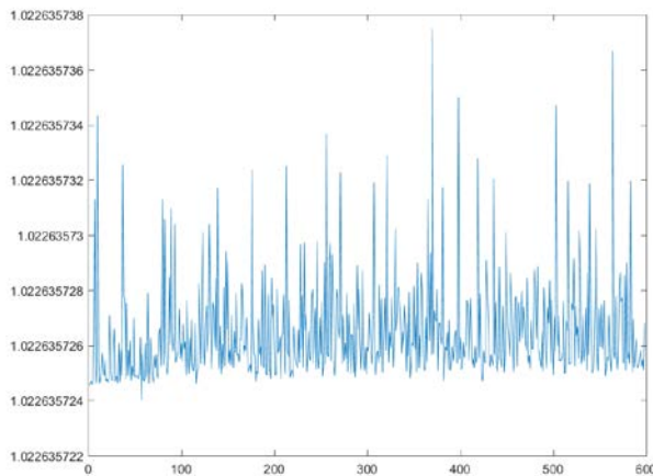
Fig. 56. Graph of field strength over time E(T) , \Delta t = 10^{-9}s
