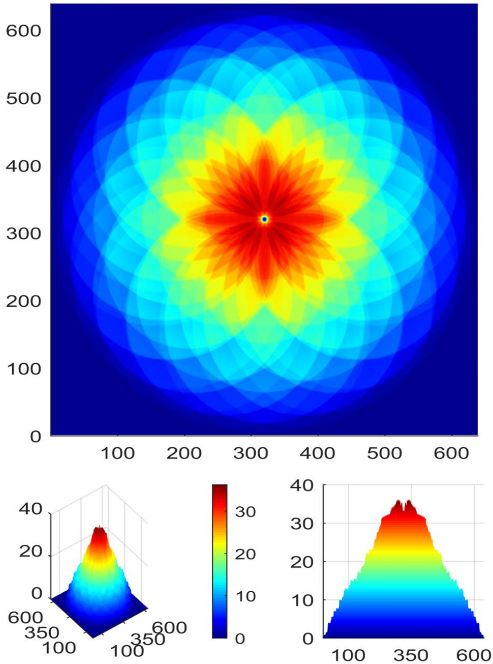
Fig.18. The distribution of the field strength E over the resonator in the 3rd stage of calculations at a height of h = 24 \mu\text{m} in different projections, range E = 0.08 \div 35.45 \text{ (V/m)}
