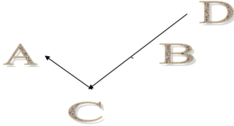
Fig. 2. Trajectory of the incident radiation DCA.
