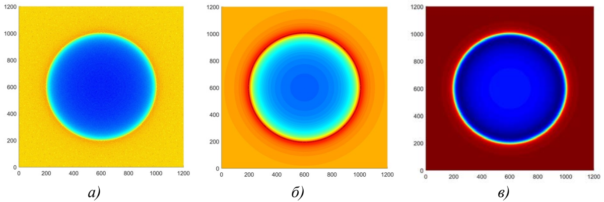
Fig. 3. Diffraction response on the 1s ring: a) \nu = 2.4 * 10^{21}\text{Hz} (gamma radiation), b) \nu = 5.5 * 10^{15}\text{Hz} (green spectrum of the Sun), c) \nu = 2.4 * 10^9\text{Hz} (Wi-Fi radiation)
