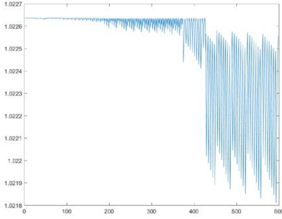
Fig. 46. Graph of field strength over time E(T) , \Delta t = 10s
