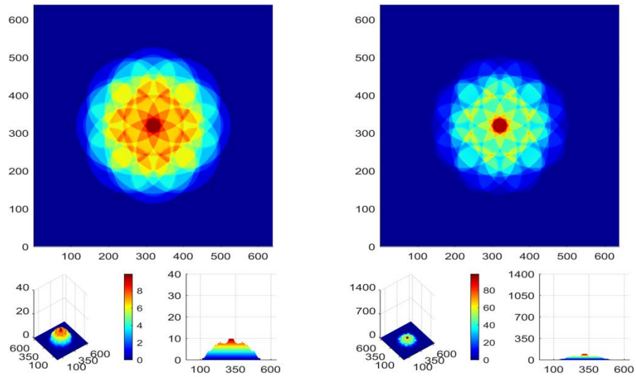
Fig.35. Strength E (on the left) and intensity I (on the right) at level 240h (5.76 mm)
