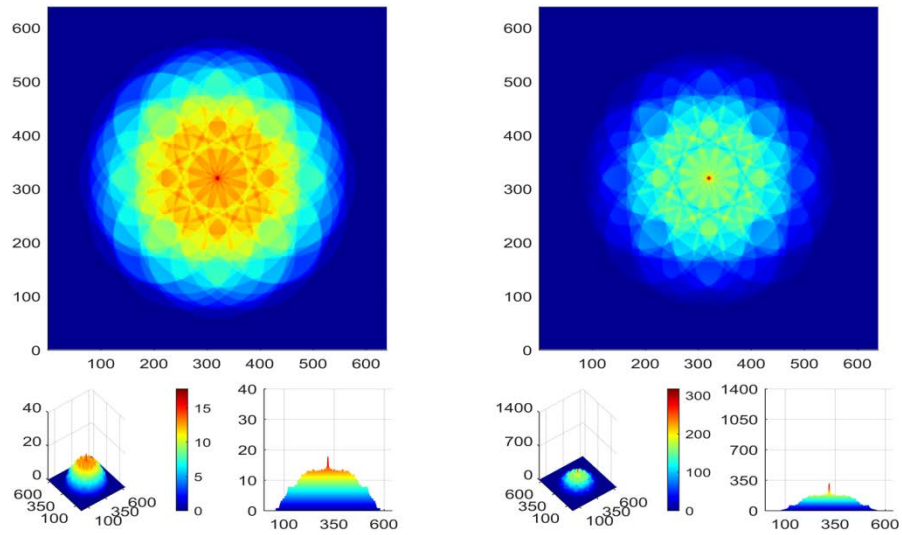
Fig.32. Strength E (on the left) and intensity I (on the right) at level 180h (4.32 mm)
