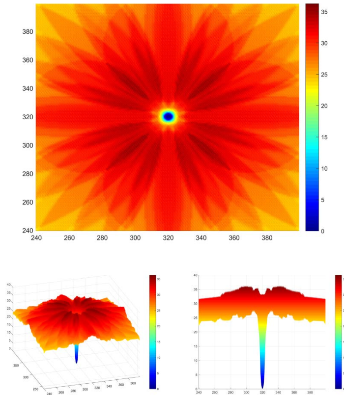
Fig. 20. The distribution of the field strength E over the resonator at a height of h = 24 \mu\text{m} in different projections, at a scale of 4:1.
