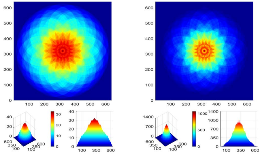
Fig.26. Strength E (on the left) and intensity I (on the right) at level 60h (1.44 mm)
