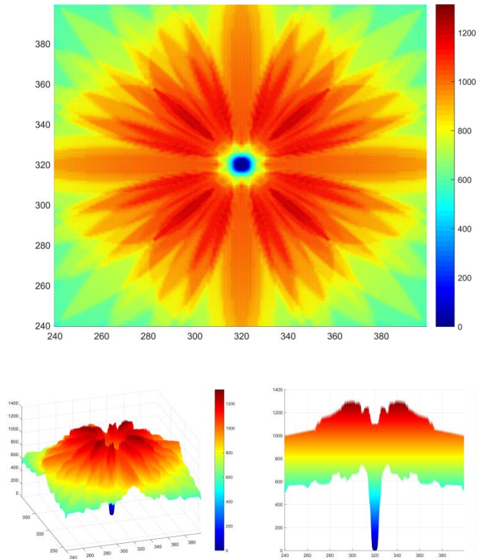
Fig. 23. The distribution of the field intensity I (W/m 2 ) over the resonator at a height of h = 24 \mu\text{m} in different projections, at a scale of 4:1.
