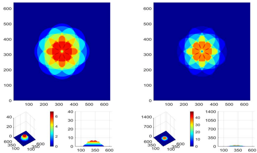
Fig.36. Strength E (on the left) and intensity I (on the right) at level 260h (6.24 mm)
