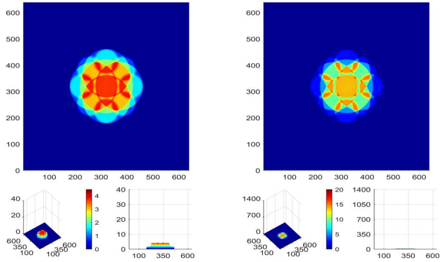
Fig.37. Strength E (on the left) and intensity I (on the right) at level 280h (6.72 mm)
