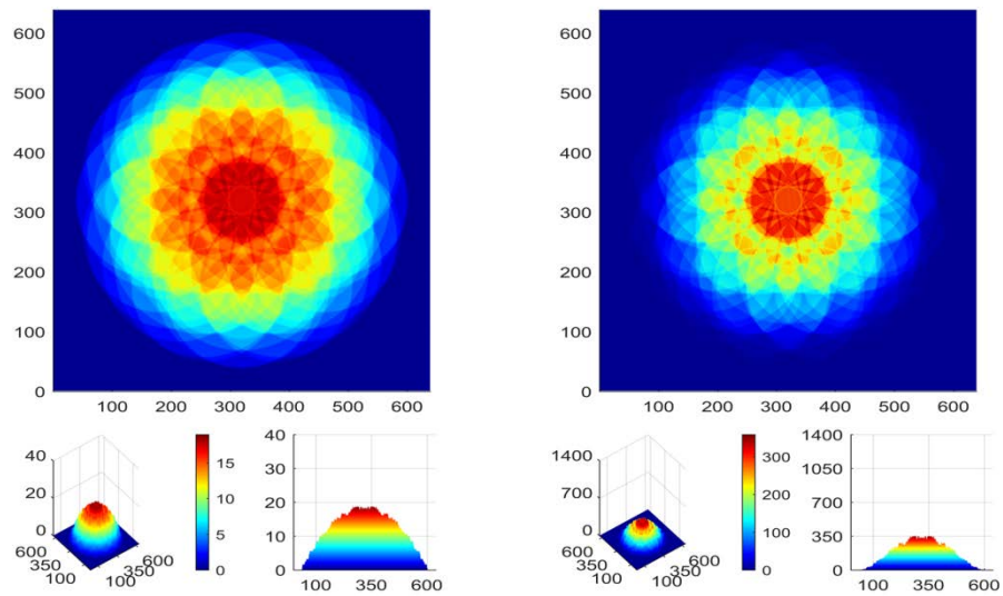
Fig.30. Strength E (on the left) and intensity I (on the right) at level 140h (3.36 mm)
