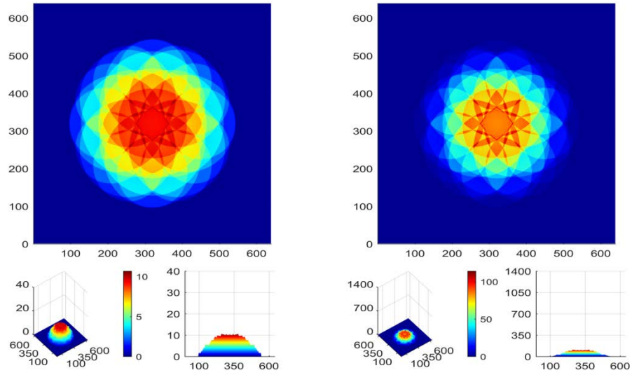
Fig.34. Strength E (on the left) and intensity I (on the right) at level 220h (5.28 mm)
