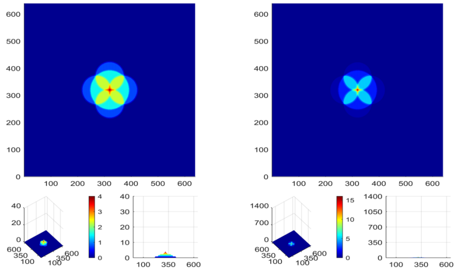
Fig.38. Strength E (on the left) and intensity I (on the right) at level 300h (7.2 mm)
