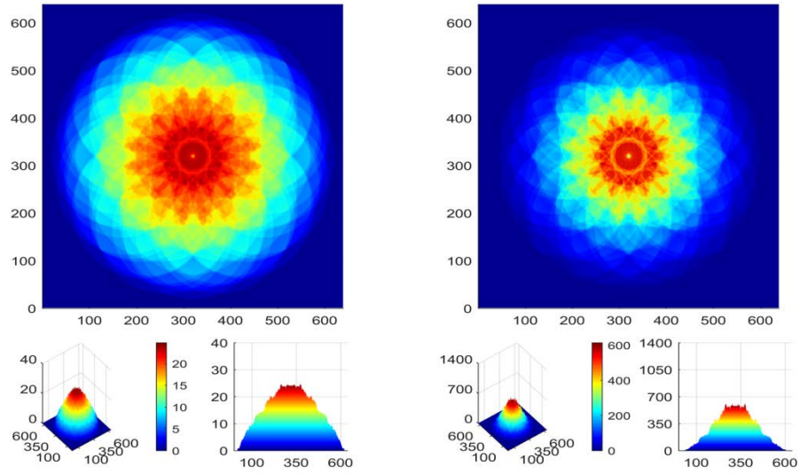
Fig.28. Strength E (on the left) and intensity I (on the right) at level 100h (2.4 mm)
